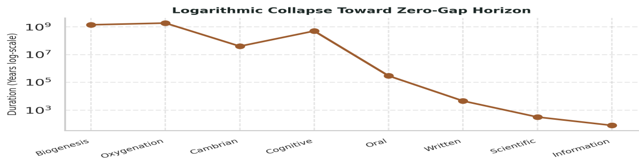
Figure 2: The logarithmic collapse of cosmic and cultural evolution Gaps (1 to 8) accelerating toward the Zero-Gap Horizon.
